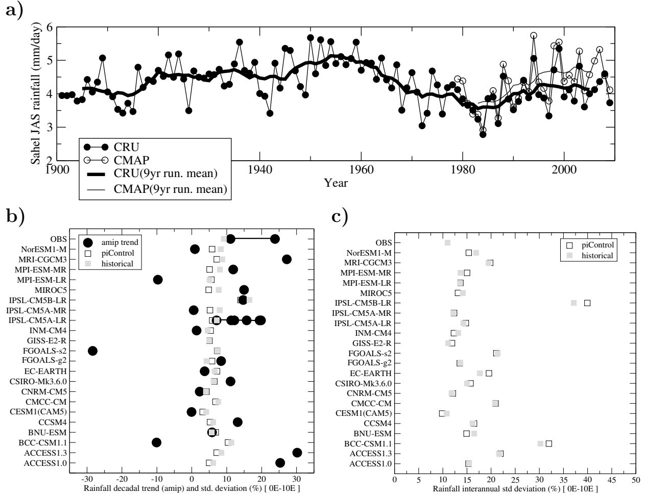
FIG. 3. a) Time evolution of raw (thin line with dots) precipitation in mm day -1 averaged over [10°N-18°N, 0°-10°E] and of its decadal component \bar{P}^9 (thick solid line), computed as the 9-year running mean of the raw index. CRU data is indicated by the thick black line and CMAP by the thin black line. b) Precipitation difference (in %) between the 9-year periods 2000–2008 and 1979–1987 for AMIP simulations (dots), and standard deviation of \bar{P}^9 in historical (open squares) and pre-industrial control (grey filled squares) experiments. The standard deviations (in %) are computed on the full period (1850–2008) for historical simulations and on the available length for pre-industrial simulations, which ranges from 250 to 1000 years depending on the model. The standard deviation has been normalized by the mean \bar{P}^9 . For observations, the square corresponds to the normalized standard deviation of CRU \bar{P}^9 while the two black circles correspond to the precipitation difference (in %) between the periods 2000–2008 and 1979–1987 in the CRU and CMAP observations. c) Standard deviation of interannual fluctuation \delta P = P - \bar{P}^9 as a fraction of the mean precipitation (in %), in pre-industrial control (grey filled squares) and historical (open squares) experiments.
