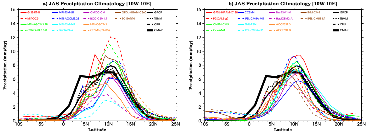
FIG. 6. Precipitation (in \text{mm day}^{-1} ) averaged over 10^\circ\text{W} - 10^\circ\text{E} , for the JAS period of the years 1979-2008 for CMIP5 simulations, and 1997-2008 for GPCP, 1998-2008 for TRMM, 1979-2008 for CRU and 1979-2008 for CMAP datasets. Each dataset is displayed using its own horizontal resolution. The left (right) panel corresponds to the warmer (colder) models over the Sahara [ 20^\circ\text{N} - 30^\circ\text{N} , 10^\circ\text{W} - 10^\circ\text{E} ].
