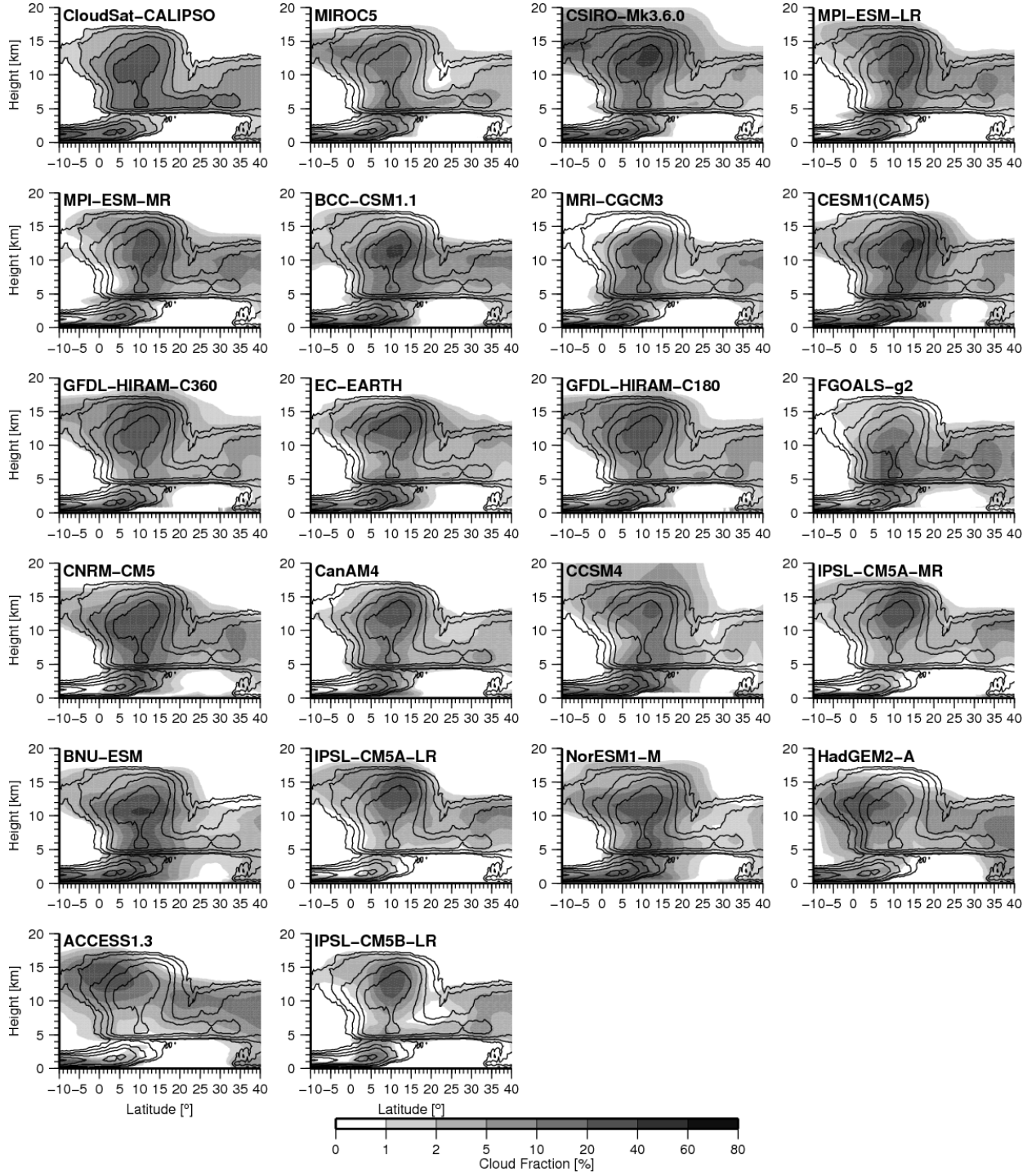
FIG. 8. Latitude-height diagrams of the cloud fraction averaged between 10^{\circ}\text{W} - 10^{\circ}\text{E} , for the period JAS of the years 2006-2010 for the CloudSat-CALIPSO data set and 1979-2008 for the models. Models are organized from the warmest one over the Sahara [ 20^{\circ}\text{N} - 30^{\circ}\text{N} , 10^{\circ}\text{W} - 10^{\circ}\text{E} ] (top left after the observation panel) to the coldest one (bottom right).
