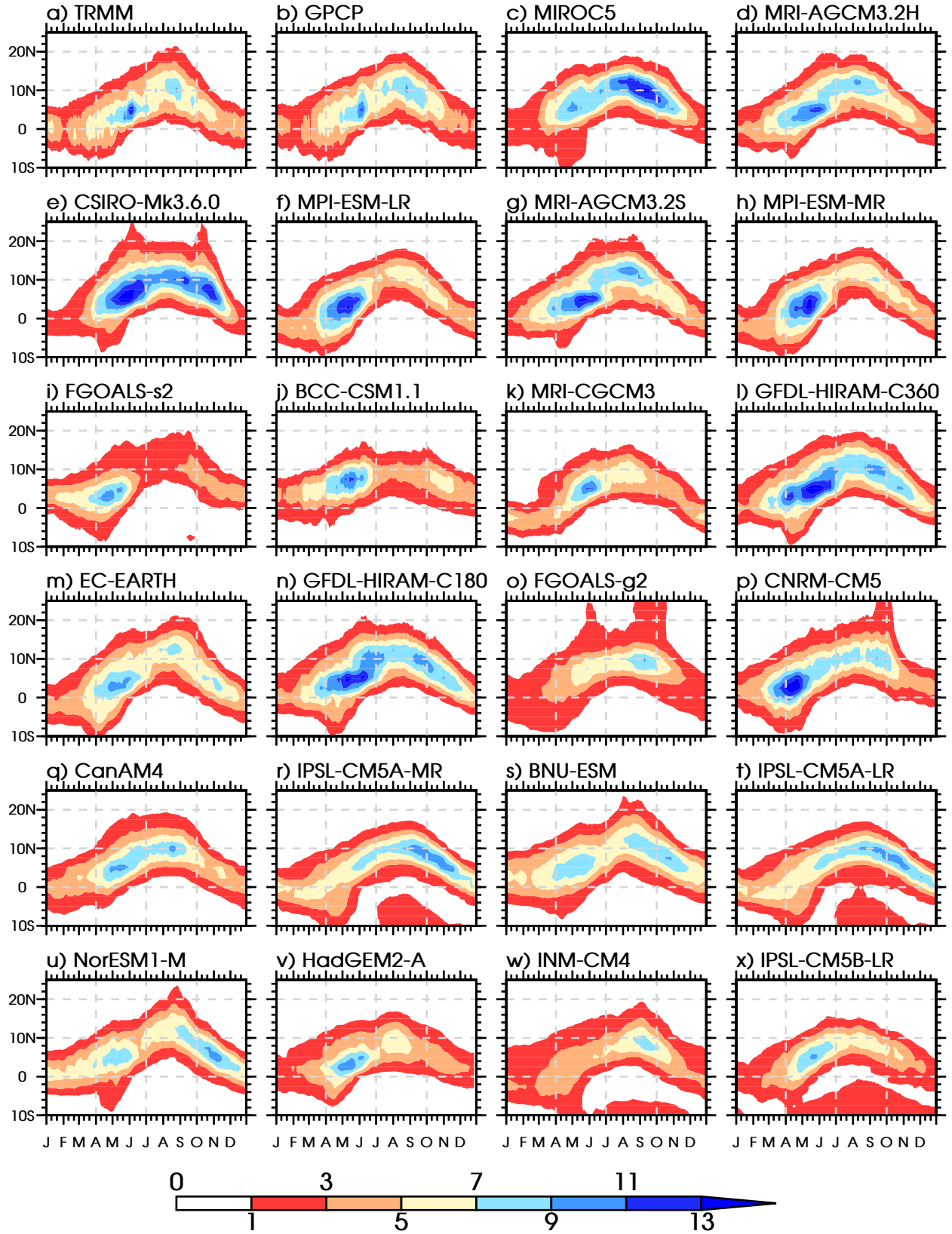
FIG. 12. Annual cycle of precipitation (in \text{mm day}^{-1} ) averaged over 10^{\circ}\text{W} – 10^{\circ}\text{E} . A 10-day running mean was performed on each dataset. Models are organized from the warmest one over the Sahara [ 20^{\circ}\text{N} – 30^{\circ}\text{N} , 10^{\circ}\text{W} – 10^{\circ}\text{E} ] (top left after the observation panel) to the coldest one (bottom right).
