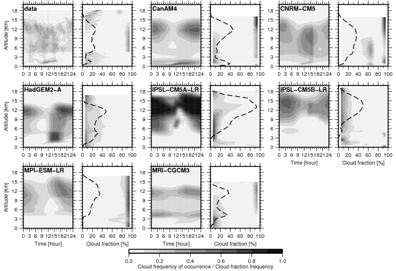
FIG. 18. As in Fig. 17 but for the August diurnal cycle of the cloud frequency of occurrence derived at the Niamey site (2.2°E-13.5°N). Observations comes from the AMF data acquired in 2006. The period 1979-2008 is used for the models. The vertical distribution of the cloud fraction is indicated on the right sub-panels. It is normalized at each level by the total cloud frequency of occurrence which is superimposed with the dashed line.
