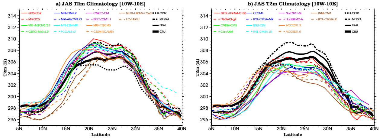
FIG. 7. 2-meter temperature (in K) averaged over 10°W-10°E, for the JAS period of the years 1979-2008 for CMIP5 simulations, reanalyses and CRU. Each dataset is displayed using its own horizontal resolution. The left (right) panel corresponds to the warmer (colder) models over the Sahara [20°N-30°N, 10°W-10°E].
