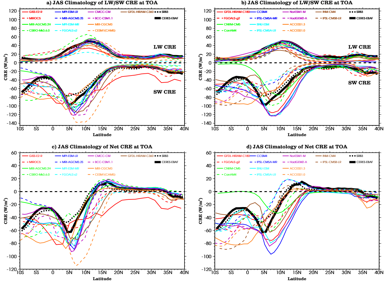
FIG. 9. a) and b) Cloud radiative effect (in \text{W m}^{-2} ) at the top of the atmosphere in the SW (negative values) and LW (positive values) bands, averaged over 10^\circ\text{W} – 10^\circ\text{E} , for the JAS period of the years 1979–2008. The left (right) panel corresponds to warmer (colder) models over the Sahara [ 20^\circ\text{N} – 30^\circ\text{N} , 10^\circ\text{W} – 10^\circ\text{E} ]. c) and d) As in a) and b) respectively, but for the net CRE at the top of the atmosphere.
