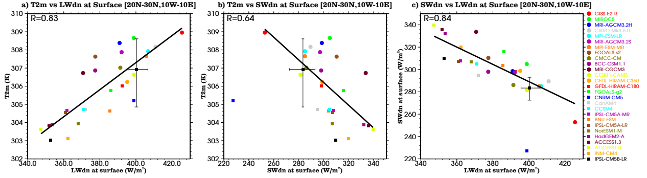
FIG. 11. a) Scatterplot of the downward longwave radiative flux at the surface (in \text{W m}^{-2} ) against the 2-meter temperature (in K). Both variables are averaged over [20°N-30°N, 10°W-10°E], for the JAS period of the years 1979-2008. A linear regression was performed and its coefficient of determination is indicated in the top-left corner. b) As in a), but for the downward shortwave radiative flux at the surface against the 2-meter temperature. Note that the linear regression was performed without the CNRM-CM5 data. c) as in b) but for the downward longwave radiative flux at the surface against the downward shortwave radiative flux at the surface (in \text{W m}^{-2} ). The black square with error bars indicates the mean obtained from observational datasets, i.e. SRB3pr, SRB3qc and CERES-EBAF for radiative fluxes, and ERAI, MERRA and CFSR for the 2-meter temperature. The warmer (colder) models are indicated with dots (filled square).
