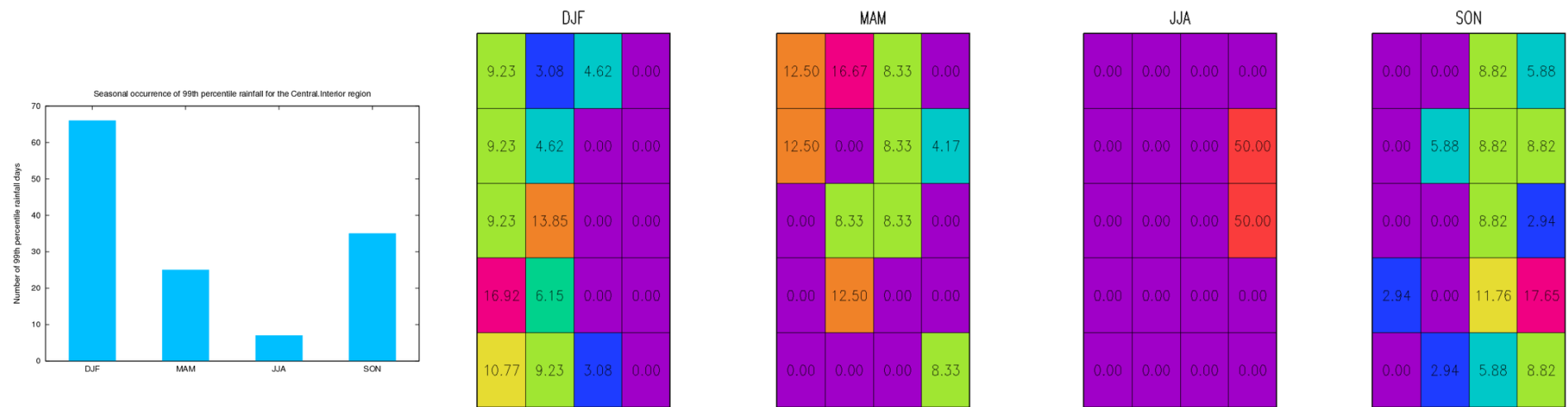
Figure 5.9. As for Figure 5.3 but for the Central Interior region
