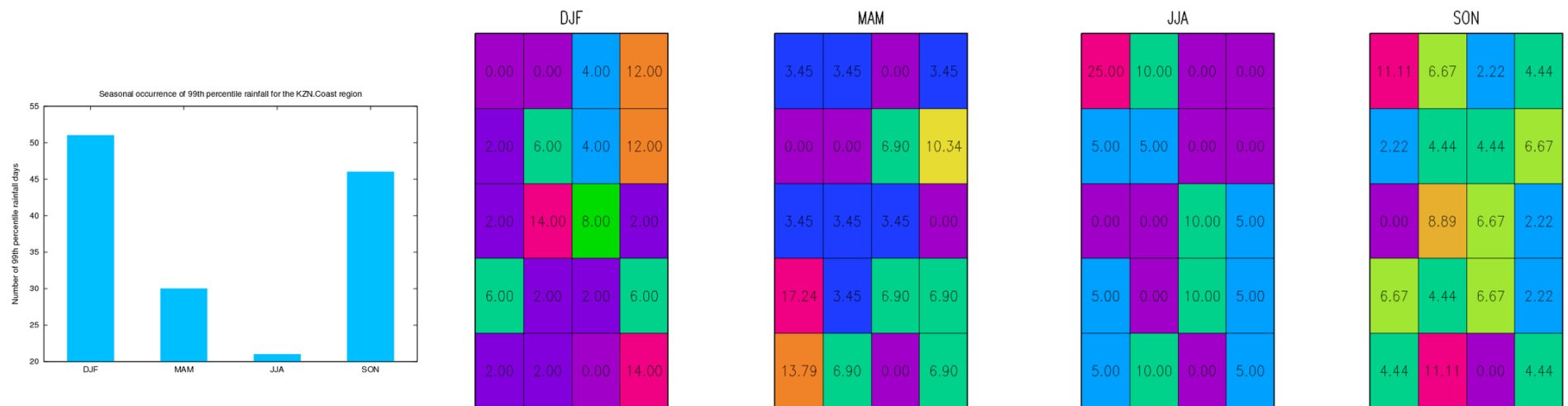
Figure 5.6. As for Figure 5.3 but for the Kwazulu-Natal region
