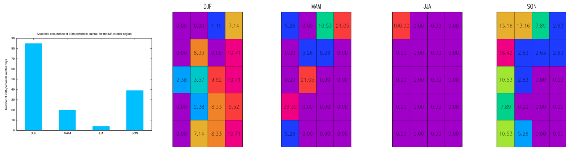
Figure 5.8. As for Figure 5.3 but for the North Eastern Interior region
