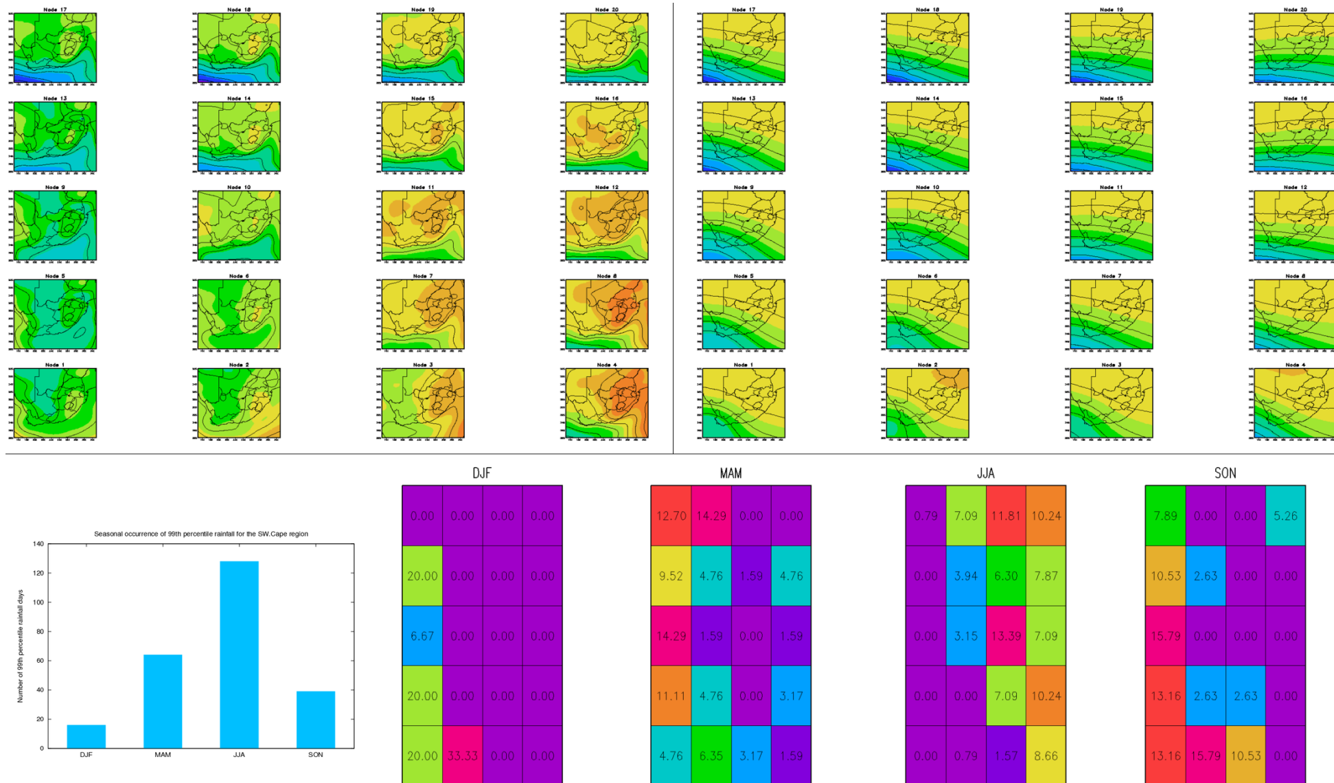
Figure 5.3. Seasonal 99th percentile SOMs of the SW Cape. The SLP and z500 archetypes are top left and right respectively. The bottom row shows the seasonal distribution of seasonal extreme rainfall on the left and frequency maps which are for the shown seasons.
