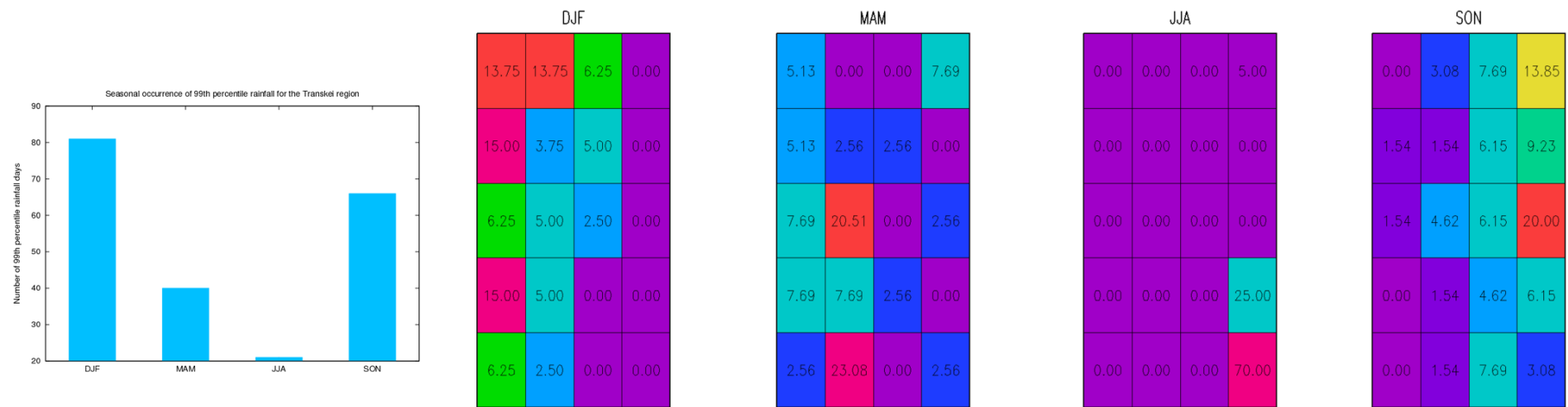
Figure 5.5. As for Figure 5.3 but for the Transkei region
