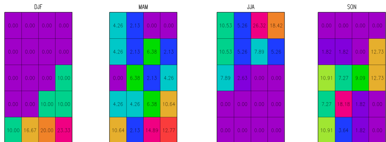
Figure 5.4. As for Figure 5.3 but for the South Coast region
